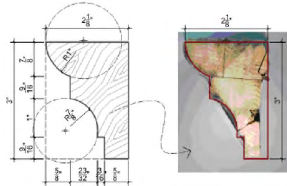
PROFILE COMPARISON WITH SAMPLE RECEIVED CROWN MOULDING "WL"
