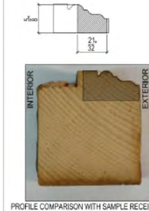
PROFILE COMPARISON WITH SAMPLE RECEIVED
