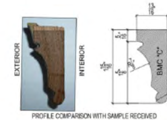
PROFILE COMPARISON WITH SAMPLE RECEIVED
